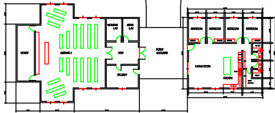
PRELIMINARY FLOOR PLAN CHAPEL - GUEST HOUSE
