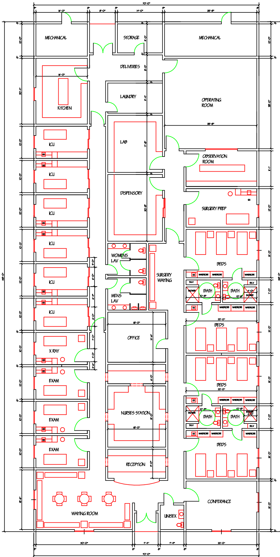
PRELIMINARY FLOOR PLAN SCALE: 1/4" = 1'-0" MAIN FACILITY - 11,060 SQUARE FEET HEART & WILL HOSPITAL - HAITI
